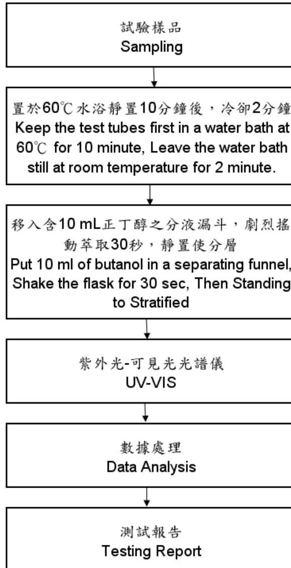
Flow Chart for Formaldehyde
